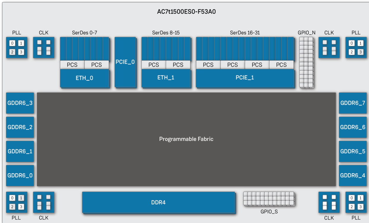
Figure 2 • Speedster7t AC7t1500 FPGA Top-Level Block Diagram
