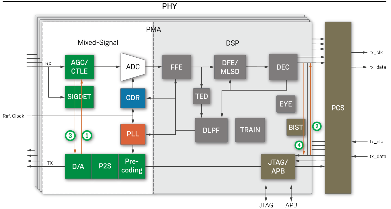
Figure 4 • Speedster7t FPGA SerDes PHY Data Loopback Modes
