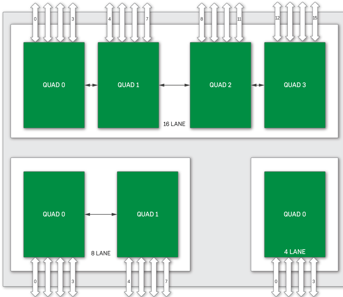
Figure 5 • SerDes Configurations
