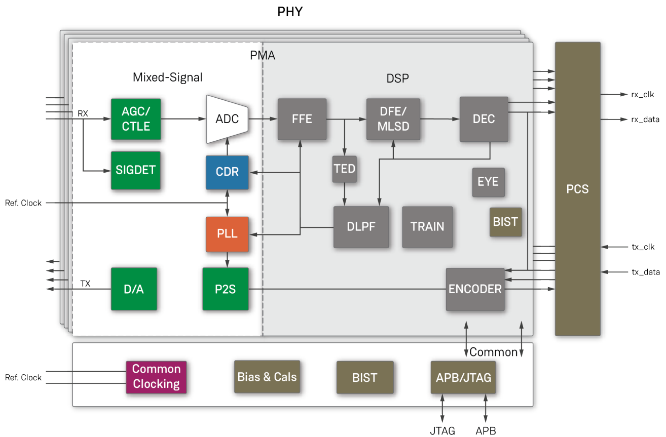
Figure 3 • Speedster7t FPGA SerDes PHY Block Diagram
