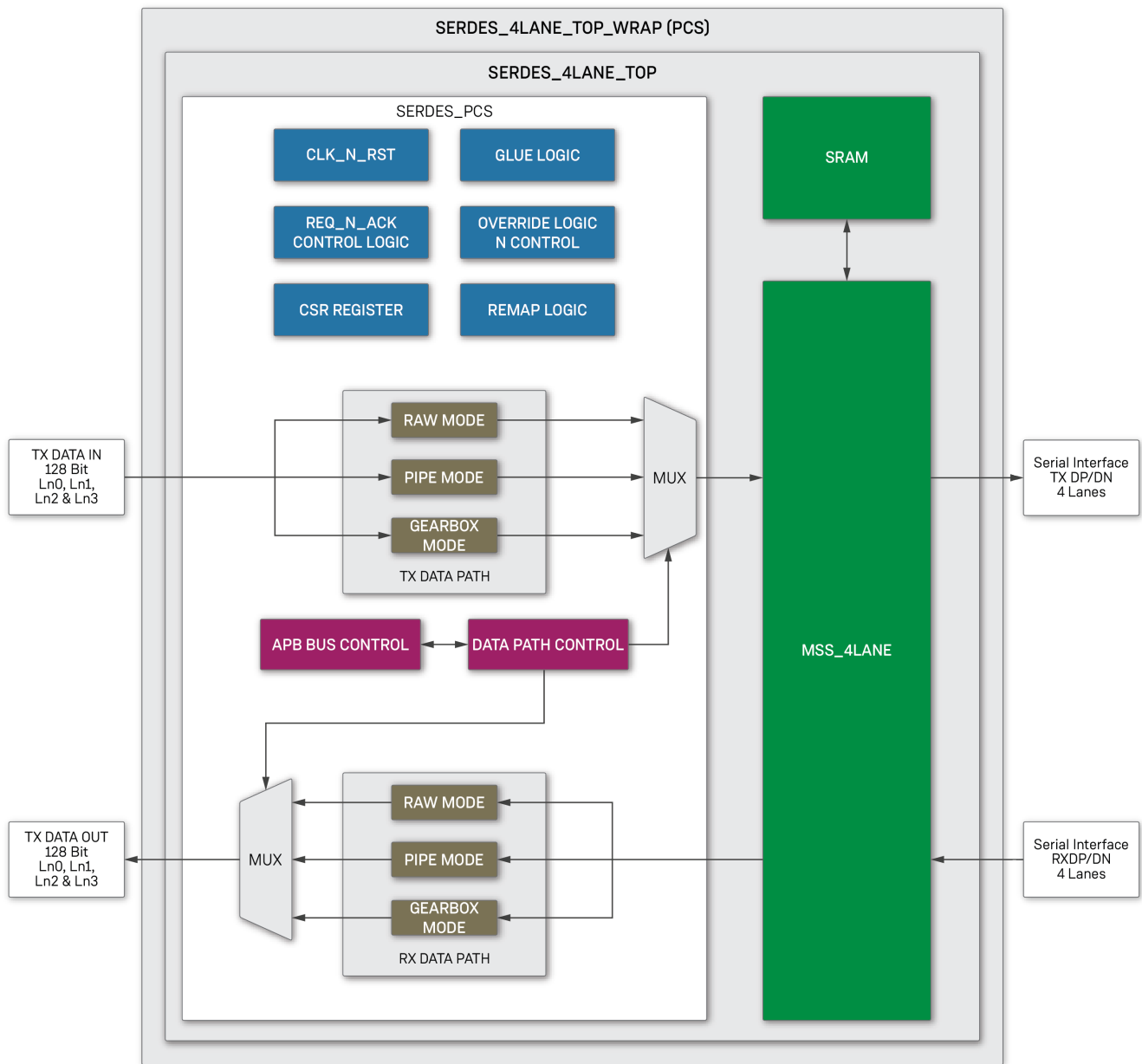
Figure 6 • PCS Modes
