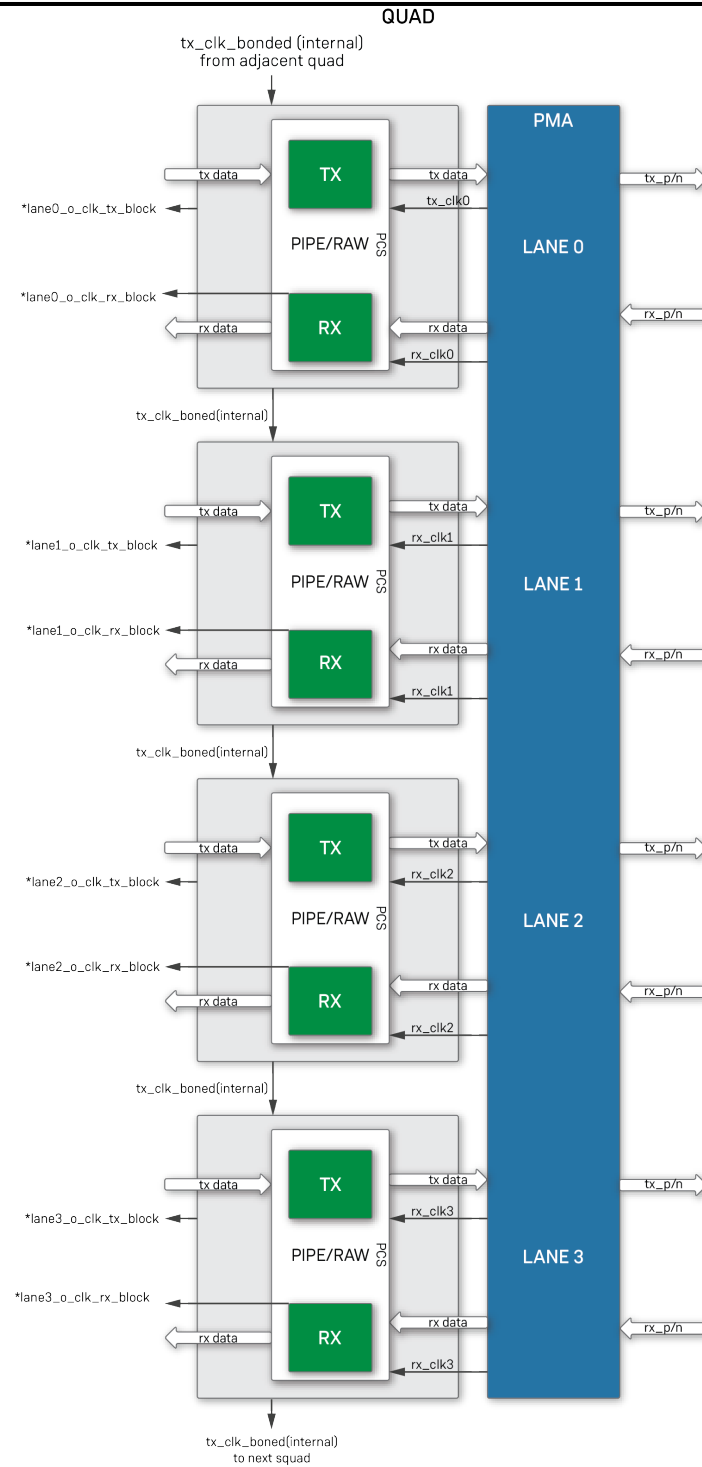
Figure 7 • Quad Transmit/Receive Path
