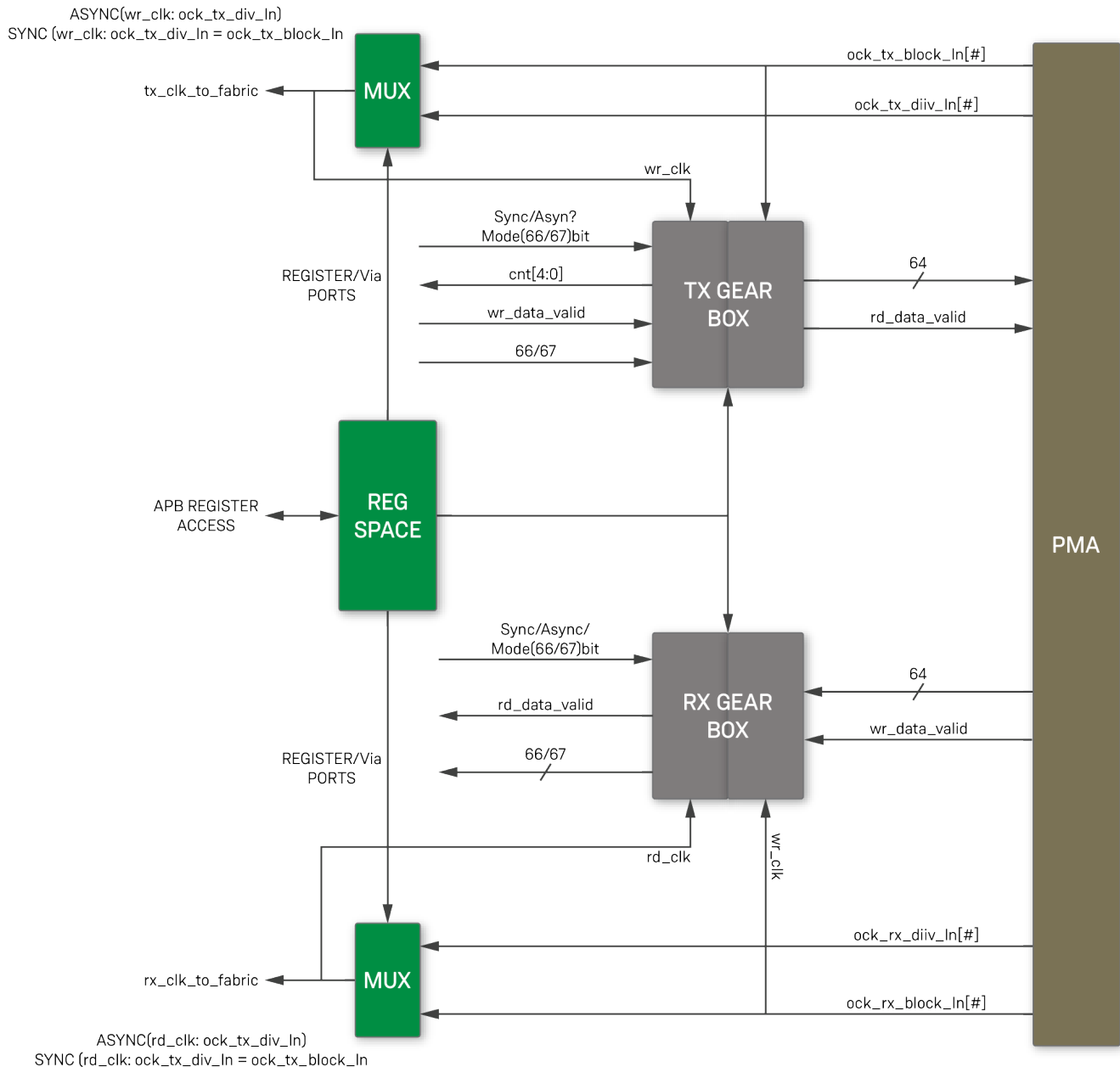
Figure 9 • Gearbox Implementation
