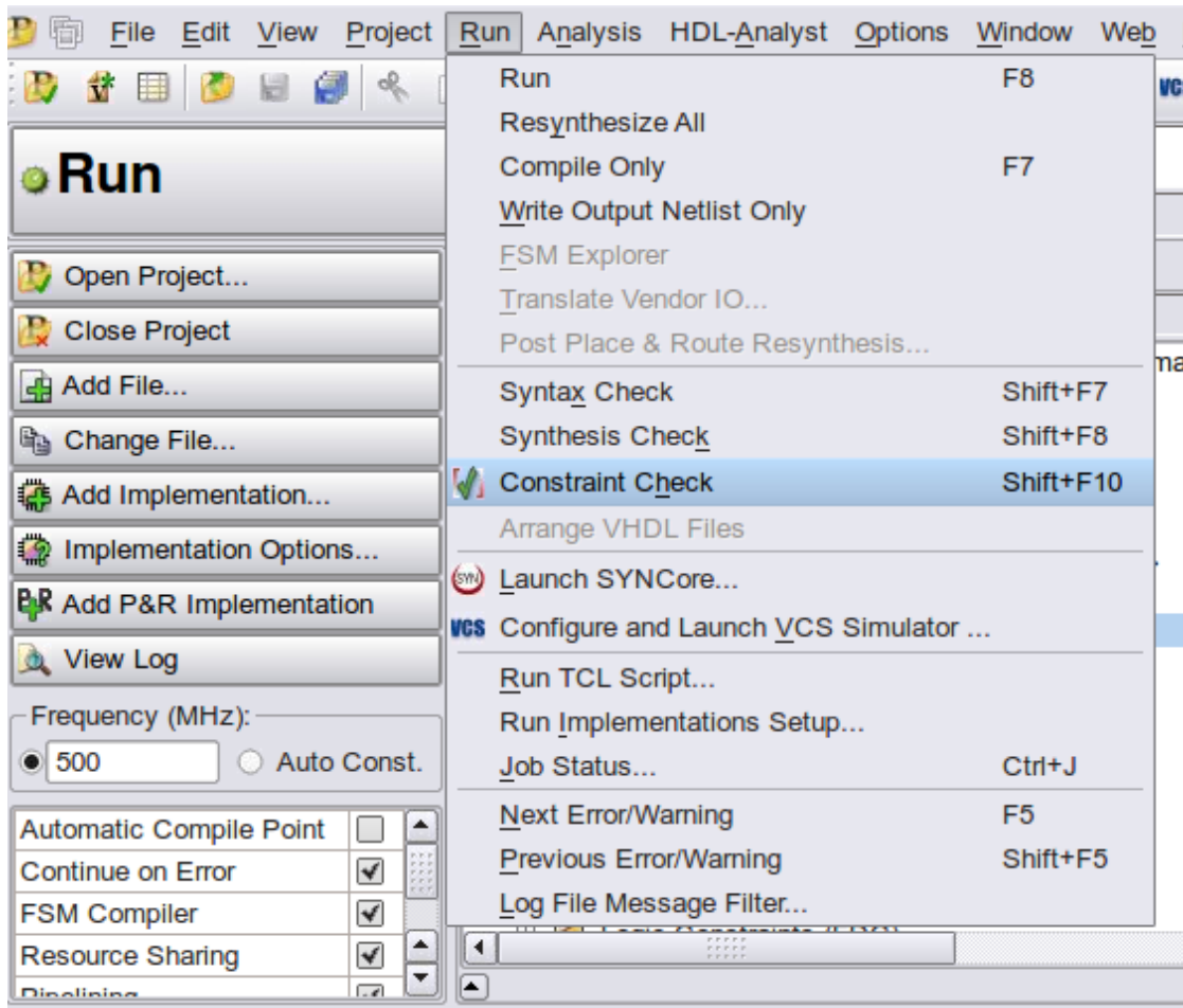
Figure 42 • Validating Constraints
