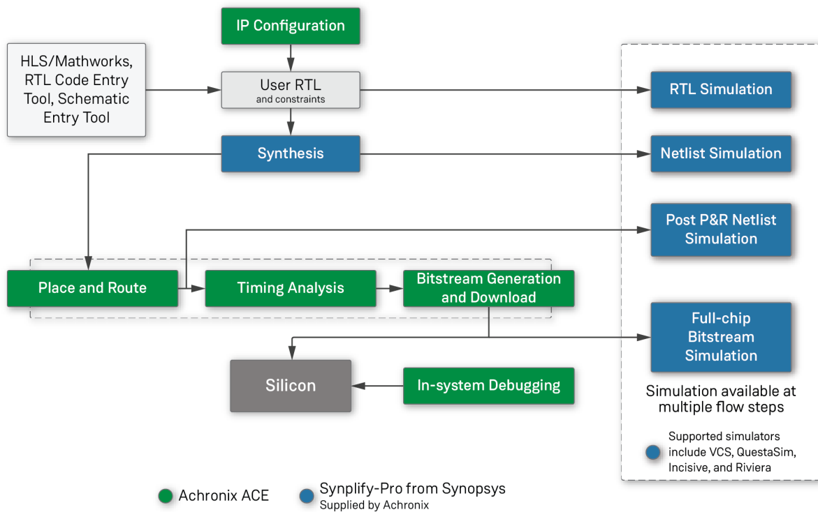
Figure 1 • Achronix Design Flow
